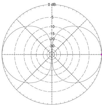
2600MHz Elevation Plot
