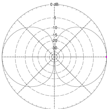
2050MHz Elevation Plot
