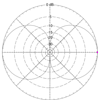
1350MHz Elevation Plot
