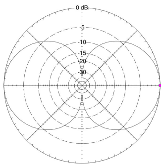
2250MHz Elevation Plot
